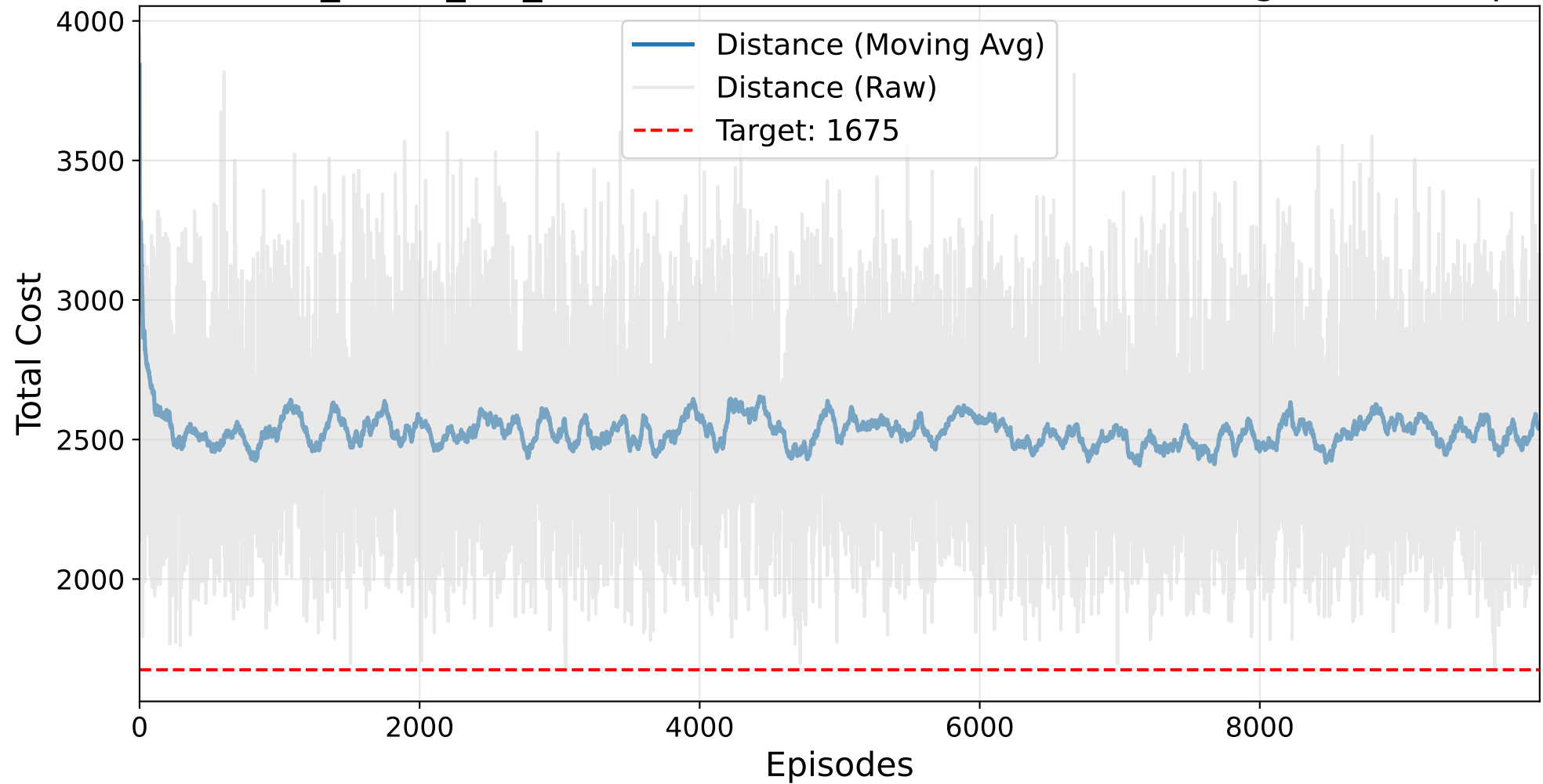
Final NO_MASK_NO_BAYESIAN Masked AutoRL-SOP Training - ESC12.sop
